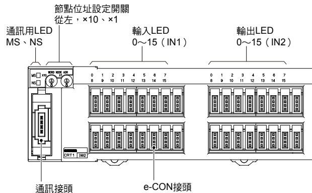
CRT1-ID32S (-1) 型、CRT1-ID32SH (-1) 型
