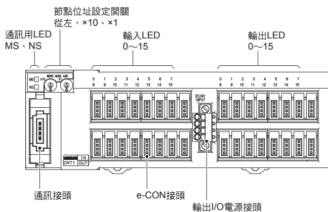
CRT1-MD32S (-1) 型、CRT1-MD32SH (-1) 型
