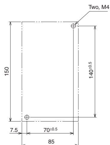
Mounting Hole Dimensions
