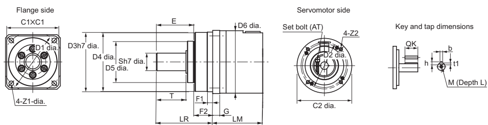
Outline Drawing 2
